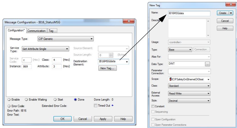
Figure 40 - Instance 869 Configuration Tab Configuration
