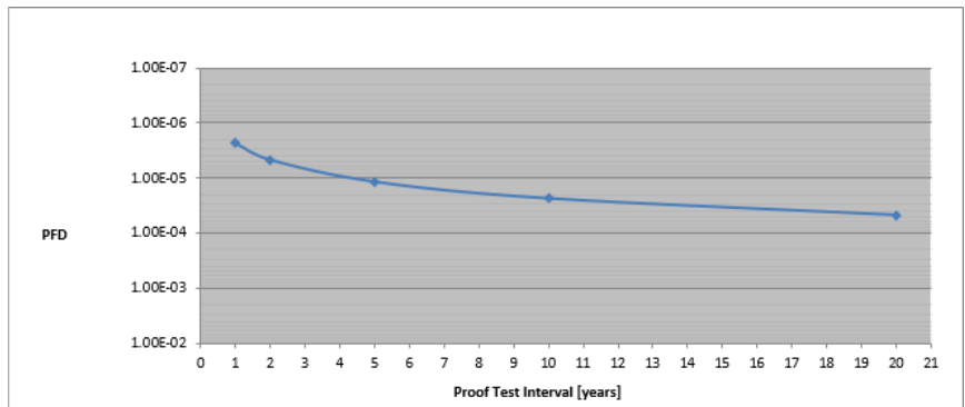
Figure 29 - PFD vs. Proof Test Interval 1732ES-IB12X0BV2, 1732ES-IB12X0B4, 1732ES-IB8X0BV4, 1732ES-IB8X0B8, 1732ES-IB16 - Single Channel Inputs
