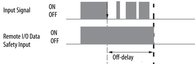
Figure 9 - Off-delay
