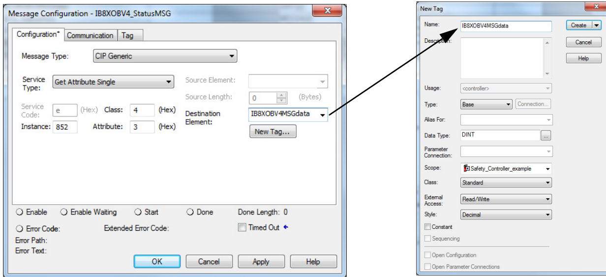
Figure 66 - Instance 852 Configuration Tab
