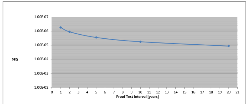
Figure 31 - PFD vs. Proof Test Interval 1732ES-IB12X0BV2, 1732ES-IB8X0BV4 - Dual Channel Outputs
